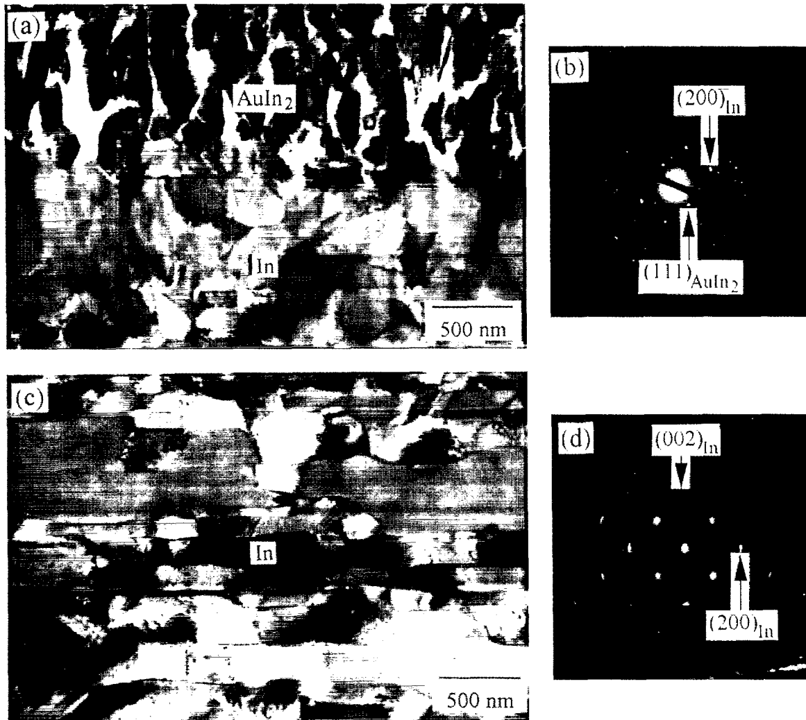
Fig. 5. (a) A cross-section TEM micrograph of the Au/In/Au microjoint after single lap tensile test. (b) The SAD pattern of an interfacial region in (a). (c) The microstructure of pure In about \sim 10 \mu\text{m} away from the In–AuIn 2 interface. (d) The SAD pattern of an area in (c).
