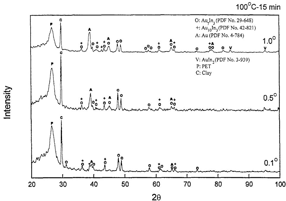
Fig. 4. Typical X-ray spectra of the Au/In microjoint hot-pressed at 100°C for 15 min, recorded at different incident angles.
