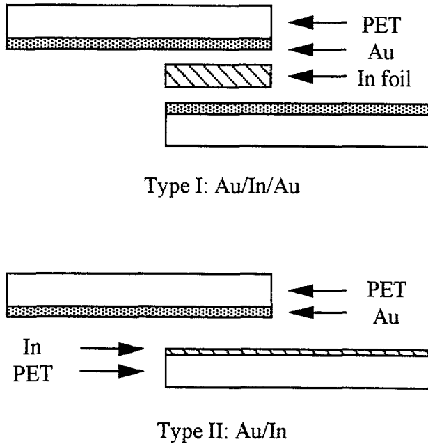
Fig. 1. Schematic of the two types of specimen geometry for single lap tensile test.
