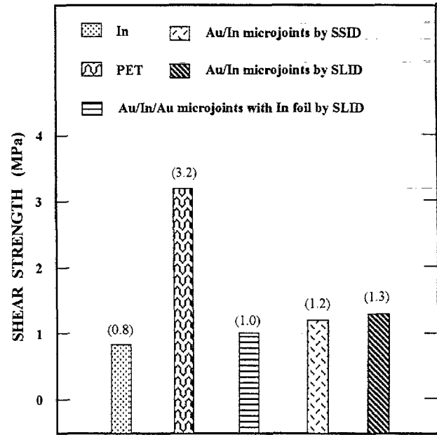
Fig. 2. A histogram showing the shear strength of the various Au–In microjoints.
