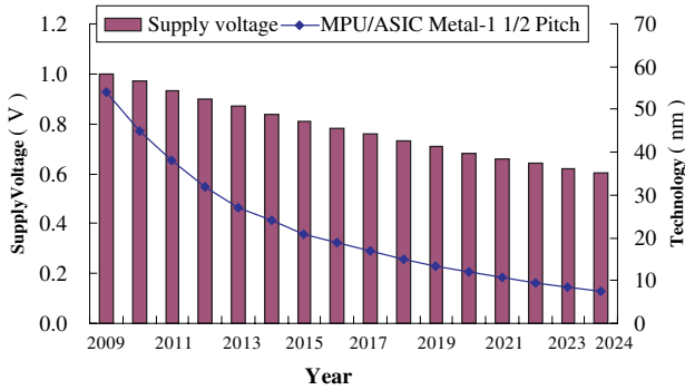
Fig. 1. A forecast of CMOS circuit for supply voltage and technologies by ITRS 2009.
