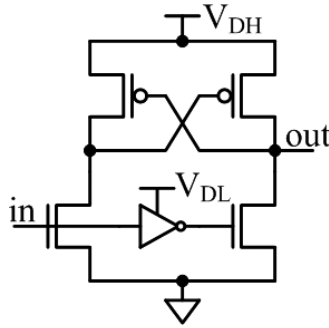
Fig. 6. Basic level converter. 50
