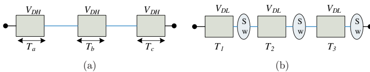
Fig. 3. Pipelined methodology.
